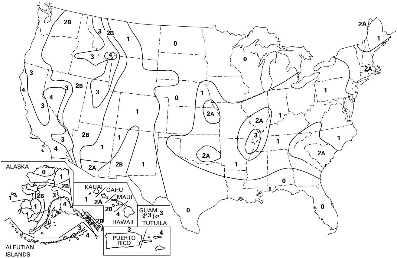
Figure 1 – 1997 Uniform Building Code Seismic Zone Map
